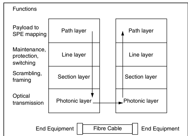
Figure 2. SONET Structure
