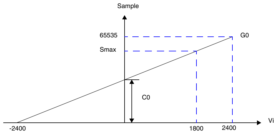
Figure 36. Offset Calculations
