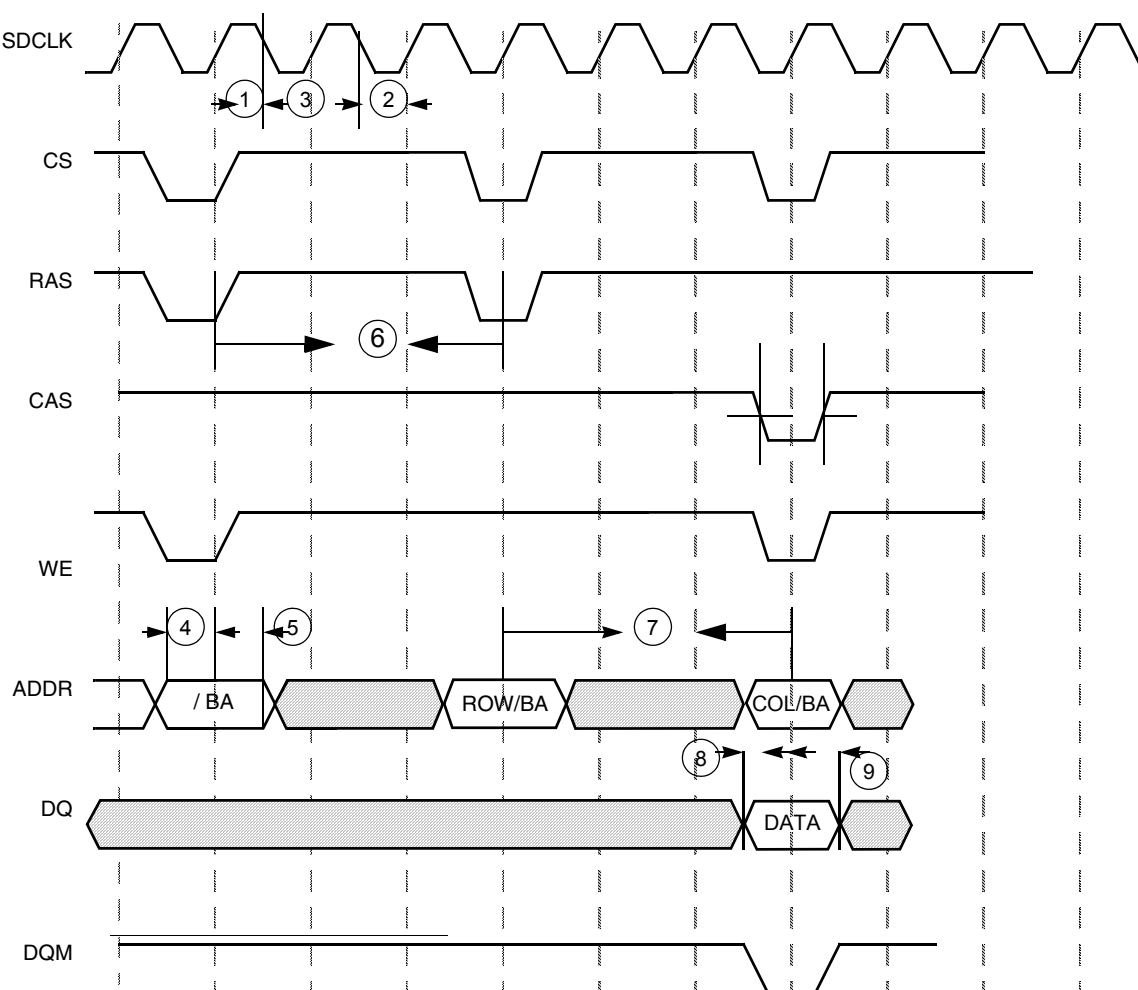
Figure 58. SDRAM/SyncFlash Write Cycle Timing Diagram
