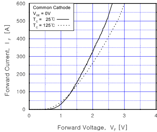
Fig 12. Forward Characteristics(diode)
