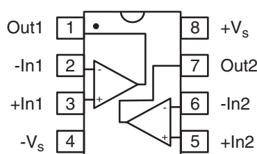
MSOP
