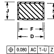
SECTION AE-AE
