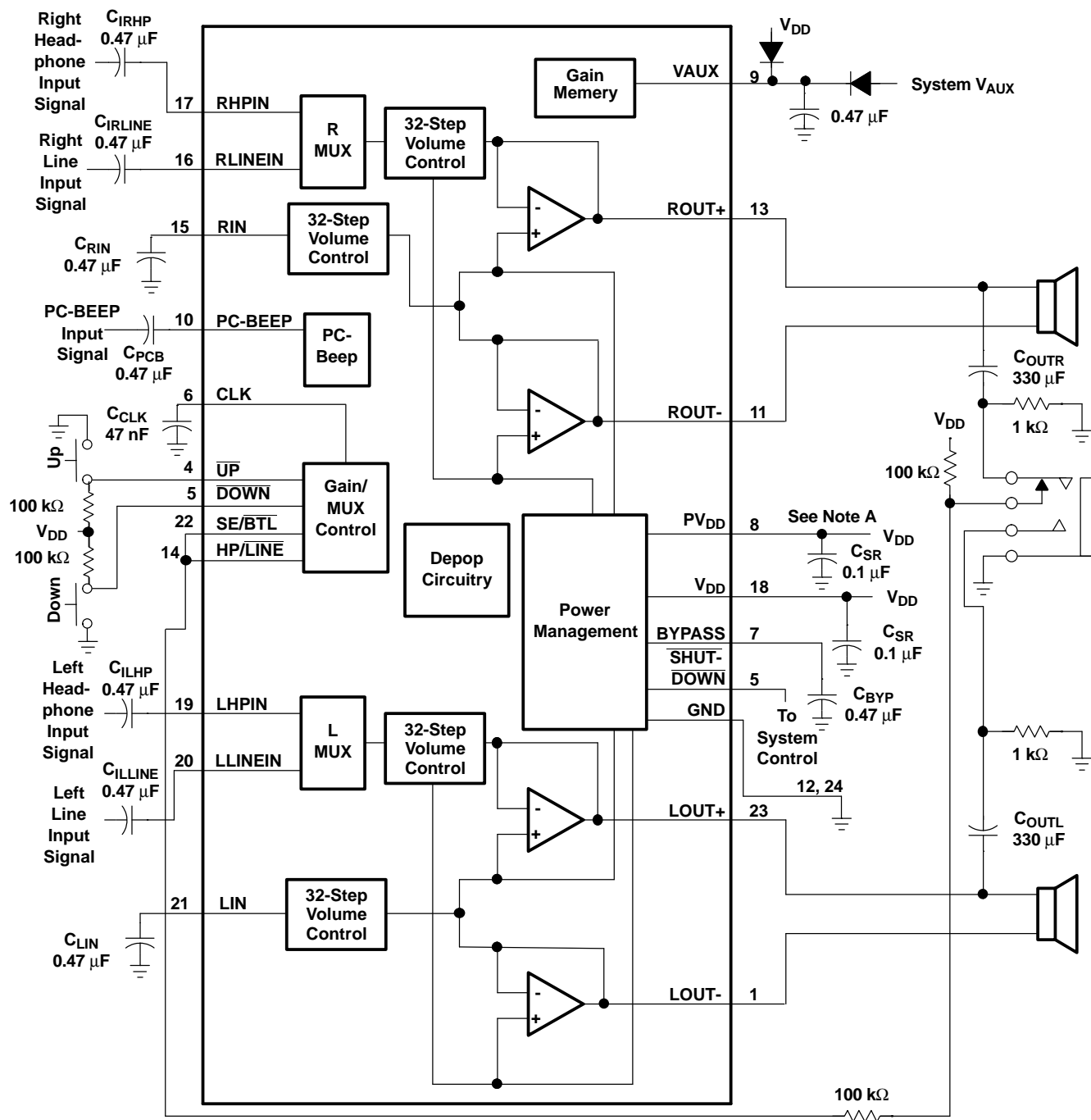
Figure 30. Typical TPA0252 Application Circuit Using Single-Ended Inputs and Input MUX
