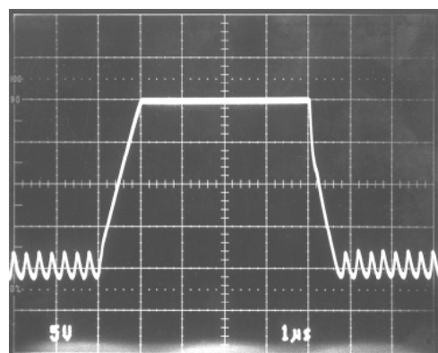
Figure 6. Large-Signal Transient Response, A_V = 1 , V_{IN} = 20\text{ V p-p} , Z_L = 2\text{ k}\Omega/200\text{ pF} , V_S = \pm 15\text{ V}
