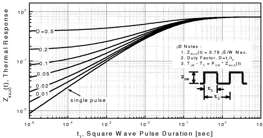
Fig 11. Thermal Response
