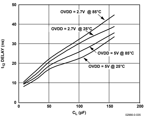
Figure 19. Typical Delay vs. Load Capacitance CL
