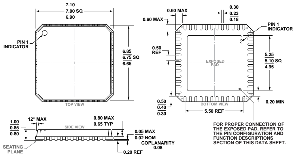
Figure 40. 48-Lead Lead Frame Chip Scale Package [LF CSP] 7 mm × 7 mm Body and 0.85 mm Package Height (CP-48-1)
