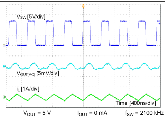
Figure 25. FPWM Mode
