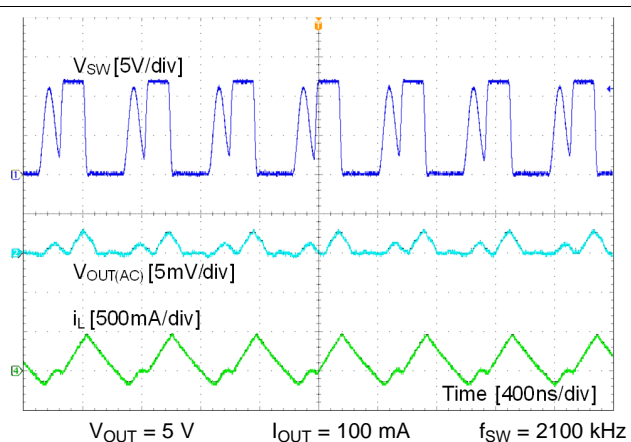
Figure 23. DCM Mode
