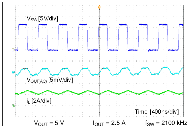
Figure 22. CCM Mode
