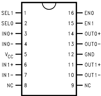
Figure 1. DS10CP152Q Pin Diagram
