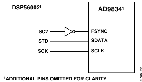
Figure 38. DSP56002 to AD9834 Interface
