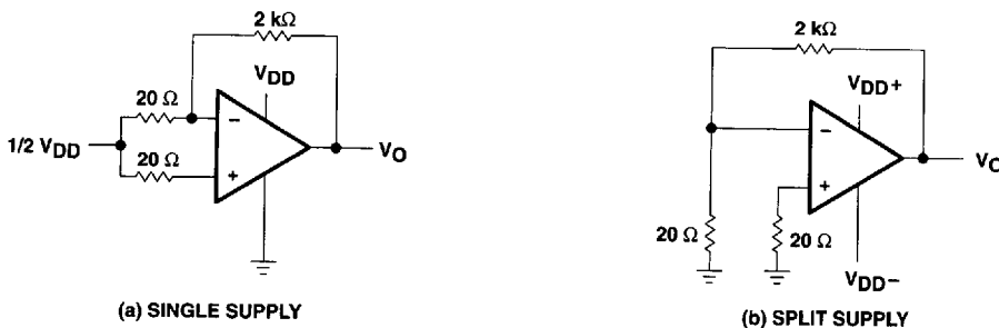
Figure 2. Noise-Test Circuit
