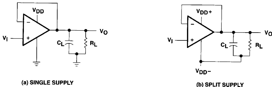
Figure 1. Unity-Gain Amplifier
