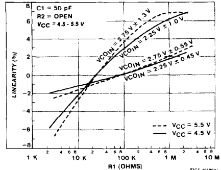
Fig. 39 - HCT7046A VCO linearity vs. R1.
