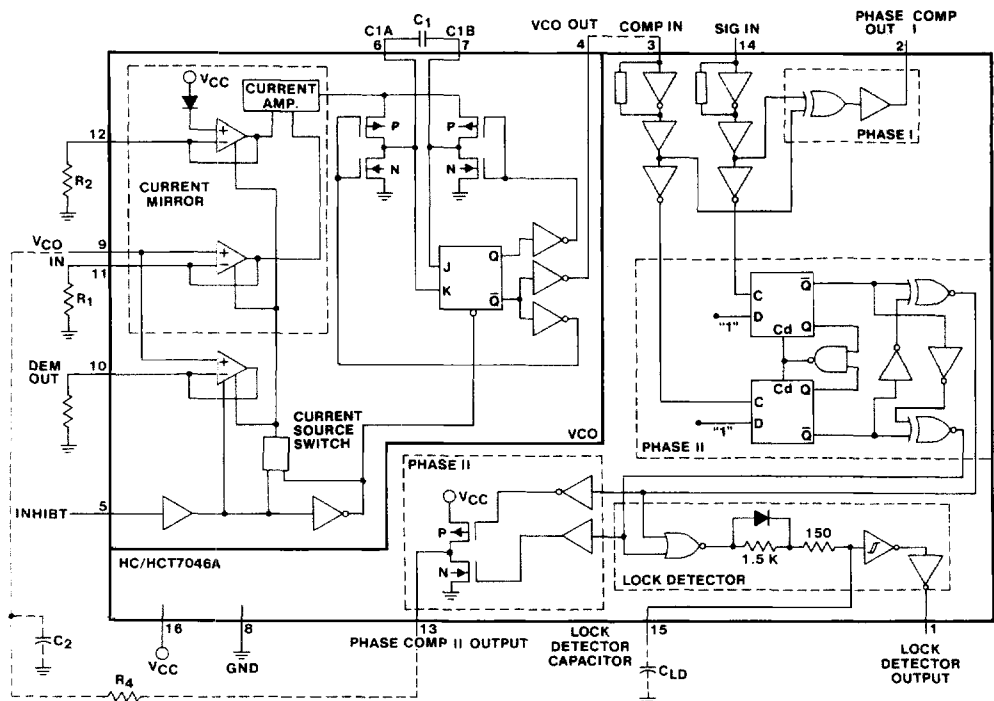
Fig. 1 - Logic diagram.
