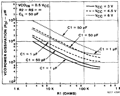
Fig. 42 - HC7046A VCO power dissipation vs. R1 (C1=50 pF, 1 μF).
