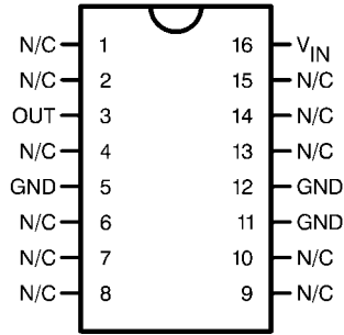
1208028 16-Lead Ceramic Surface-Mount Package (Top View) Order Part Number LM3940WG-3.3-QML 5962-9688401QXA NSC Drawing Number WG16A
