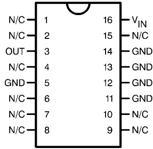
1208027 16-Lead Ceramic Dual-in-Line Package (Top View) Order Part Number LM3940J-3.3-QML 5962-9688401QEA NSC Drawing Number J16A
