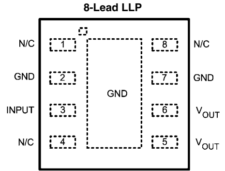
(Top View) Order Part Number LM3940LD-3.3 NSC Drawing Number LDC08A
