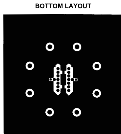
FIGURE 3. EVALUATION BOARD LAYOUT FOR SOIC
