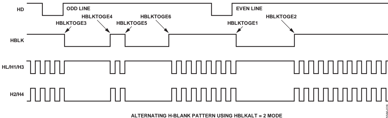
Figure 30. HBLK Odd/Even Alternation Using HBLKALT = 2
