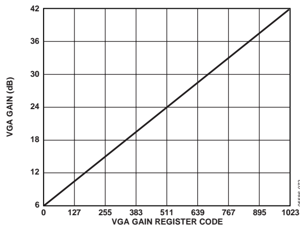
Figure 73. VGA Gain Curve
