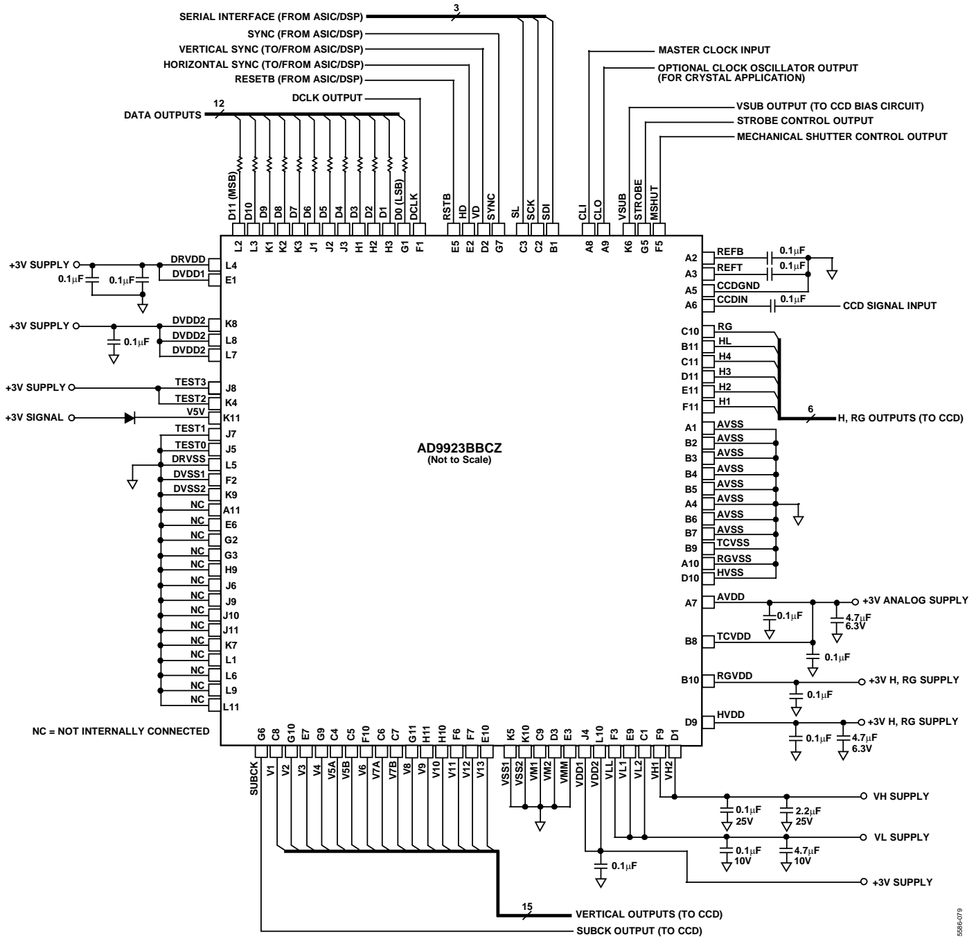
Figure 81. AD9923BBCZ Typical Circuit Configuration
