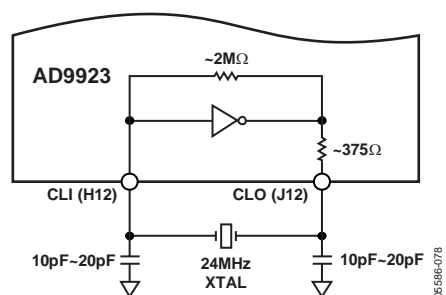
Figure 79. Crystal Driver Application
