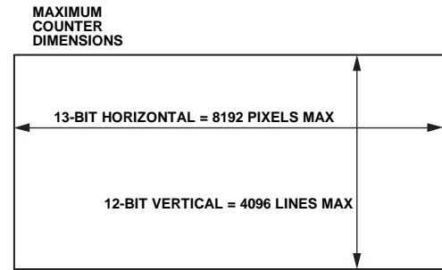
Figure 15. Vertical and Horizontal Counters
