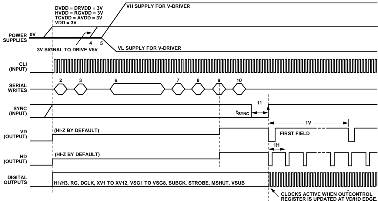
Figure 74. Recommended Power-Up Sequence and Synchronization, Master Mode
