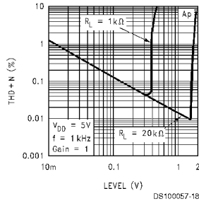
Microphone THD+N vs Output Level
