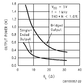
Output Power vs Load
