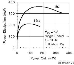
Power Dissipation, Single-Ended
