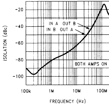
EL2257C Channel to Channel Isolation vs Frequency
