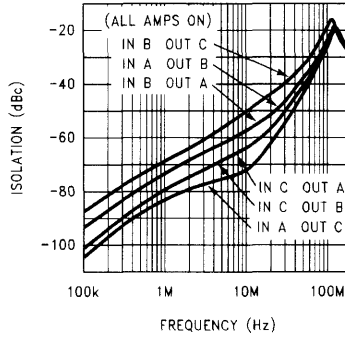
EL2357C Channel to Channel Isolation vs Frequency
