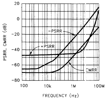
PSSR and CMRR vs Frequency
