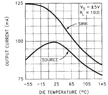
Output Current vs Die Temperature
