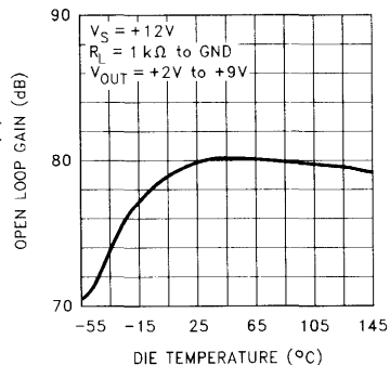
Open Loop Voltage Gain vs Die Temperature
