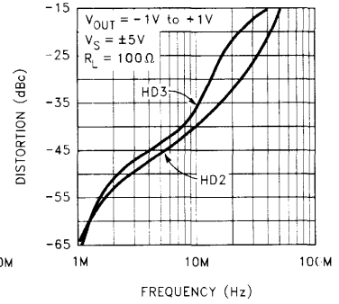
2nd and 3rd Harmonic Distortion vs Frequency
