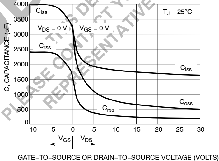
Figure 7. Capacitance Variation
