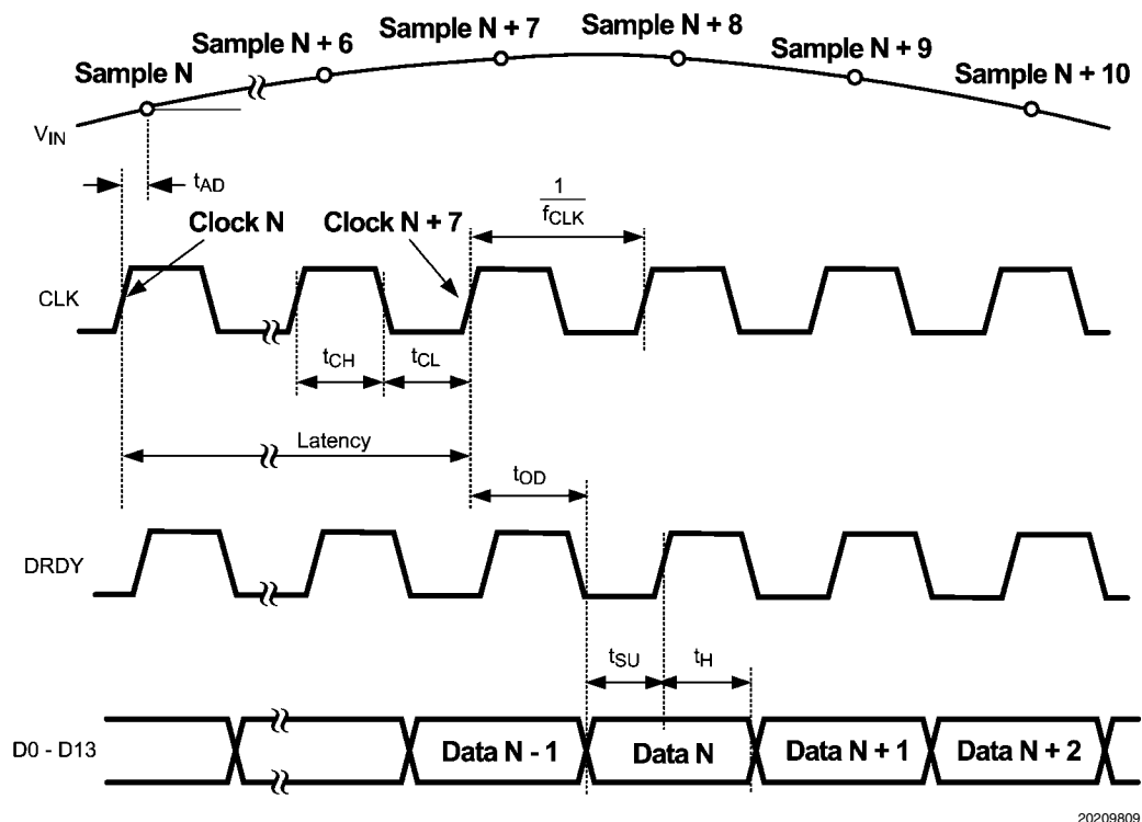
FIGURE 1. Output Timing
