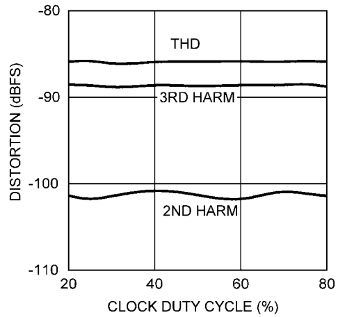
Distortion vs. Clock Duty Cycle, DCS Enabled
