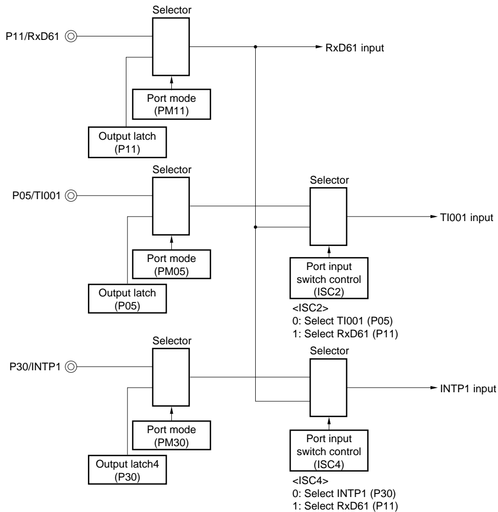
Figure 14-5. Port Configuration for LIN Reception Operation: 78K0/FE2, 78K0/FF2 (UART61)
