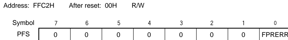
Figure 24-25. Format of Flash Status Register (PFS)
