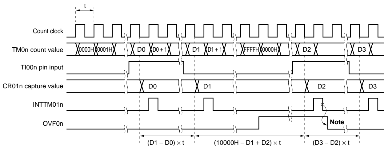
Figure 7-39. Timing of Pulse Width Measurement Operation with Free-Running Counter and One Capture Register (with Both Edges Specified)
