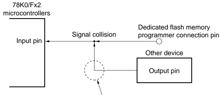
Figure 24-15. Signal Collision (Input Pin of Serial Interface)
