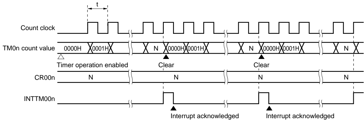
Figure 7-32. Timing of Interval Timer Operation
