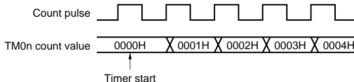
Figure 7-57. Start Timing of TM0n Count
