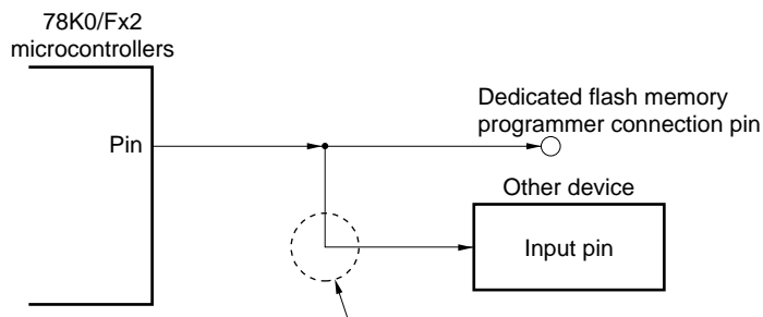
Figure 24-16. Malfunction of Other Device
