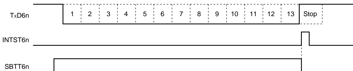
Figure 14-31. SBF Transmission
