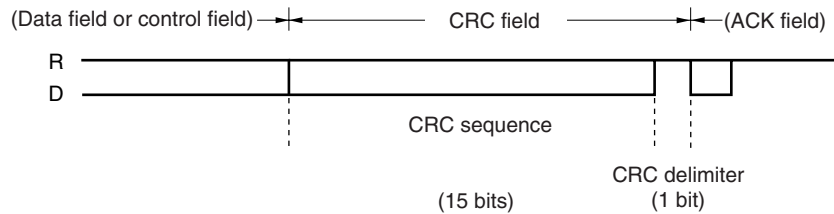
Figure 16-10. CRC Field
