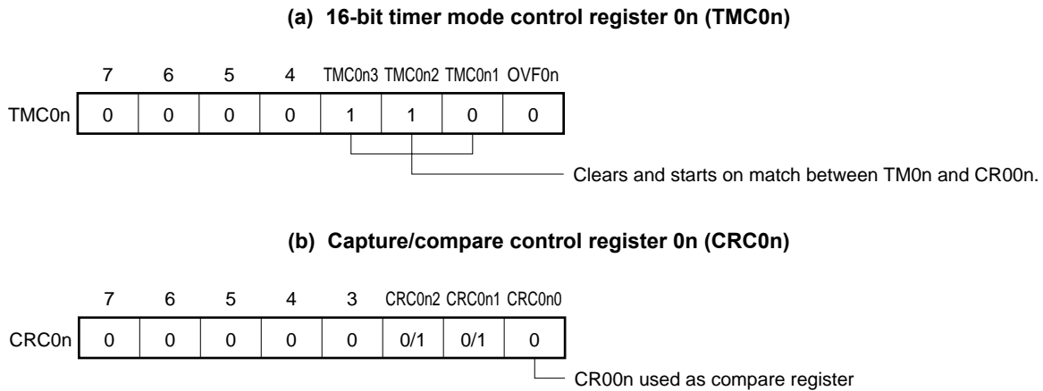
Figure 7-49. Control Register Settings in Square-Wave Output Mode (1/2)
