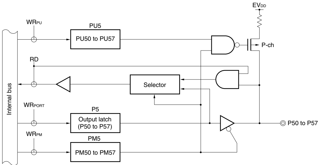
Figure 5-12. Block Diagram of P50 to P57
