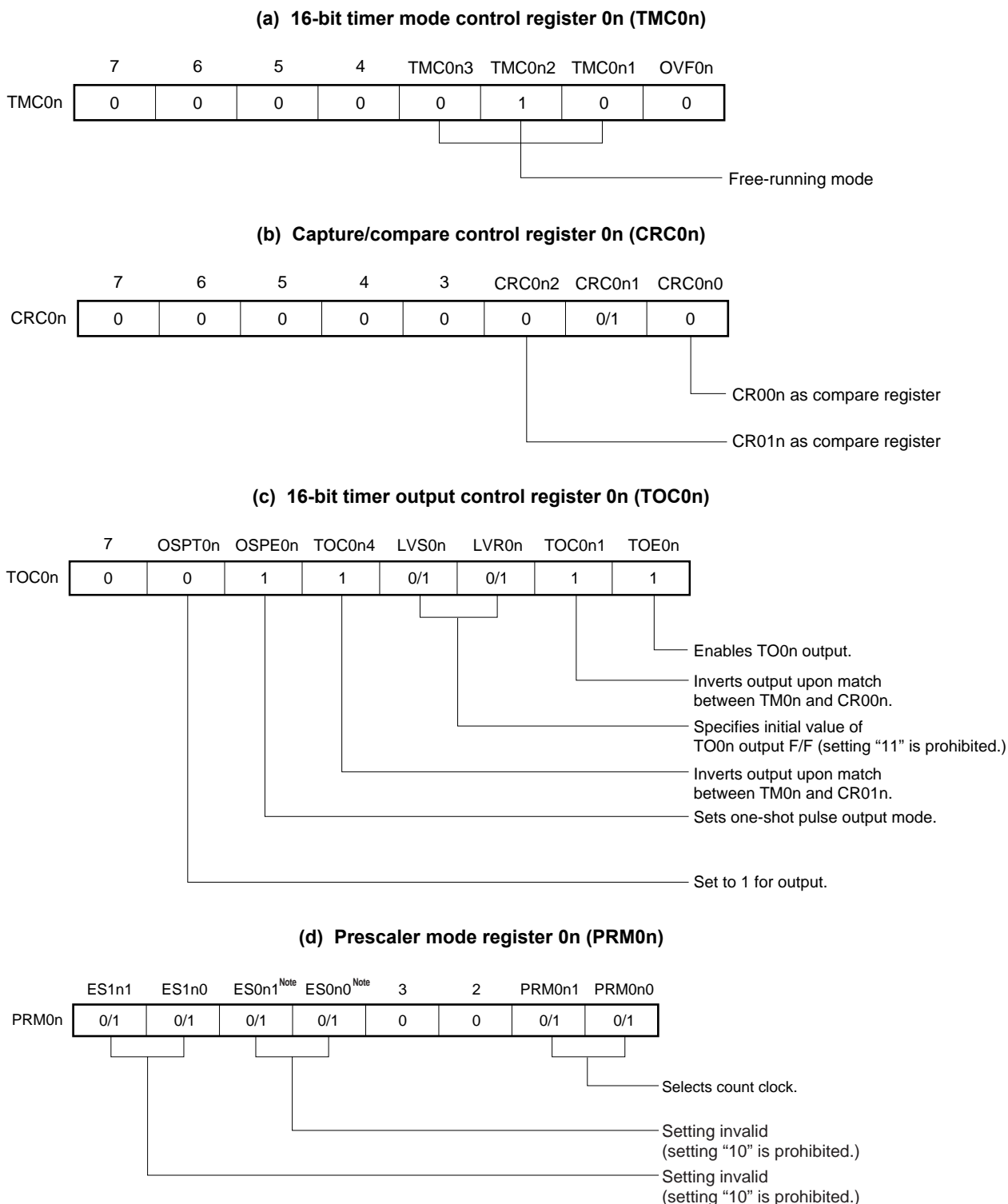
Figure 7-51. Control Register Settings for One-Shot Pulse Output with Software Trigger
