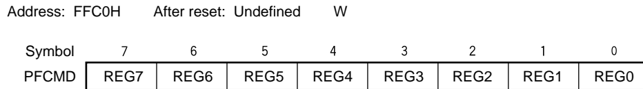
Figure 24-24. Format of Flash Protect Command Register (PFCMD)
