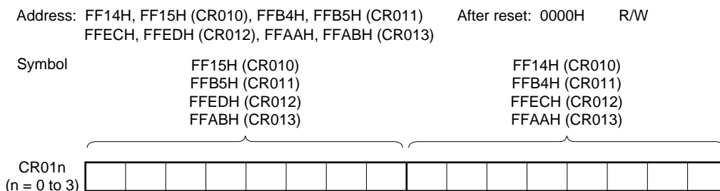
Figure 7-9. Format of 16-Bit Timer Capture/Compare Register 01n (CR01n)
