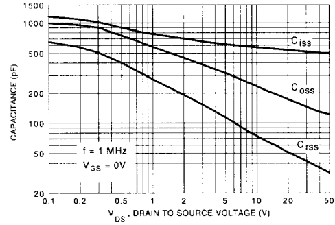
Figure 9. Capacitance Characteristics
