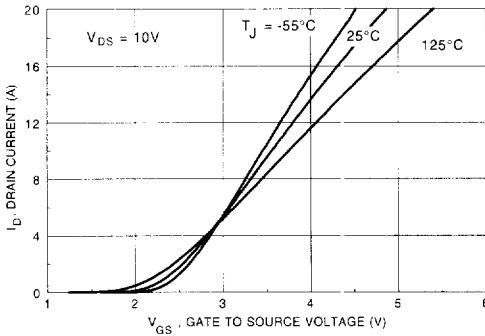
Figure 5. Transfer Characteristics
