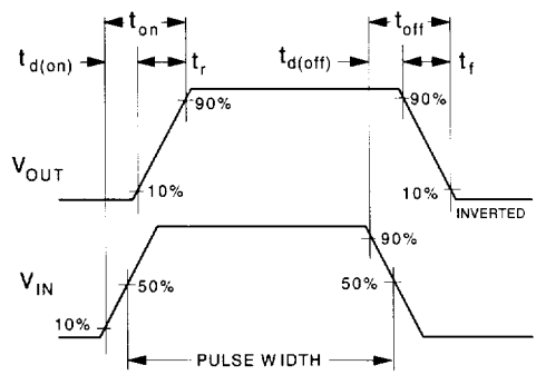
Figure 12. Switching Waveforms
