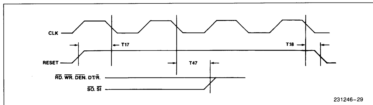
Figure 28. RESET Timing
