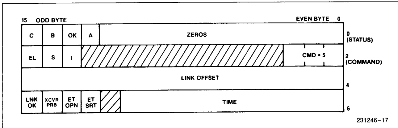
Figure 17. The TDR Command Block
