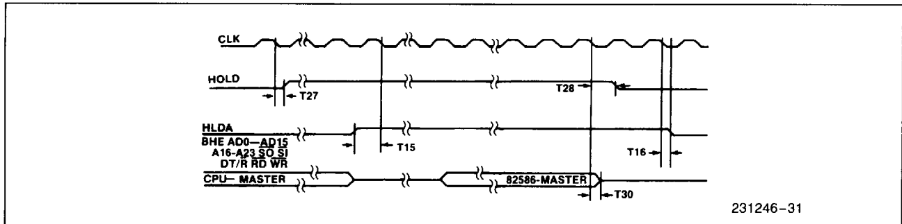
Figure 30. HOLD/HLDA Timing Relative to CLK
