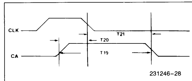
Figure 27. CA Input Timing
