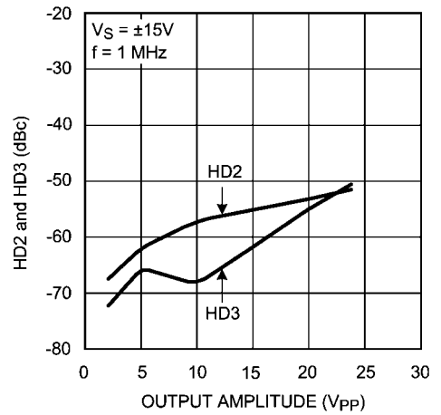
Harmonic Distortion with 100Ω Load
