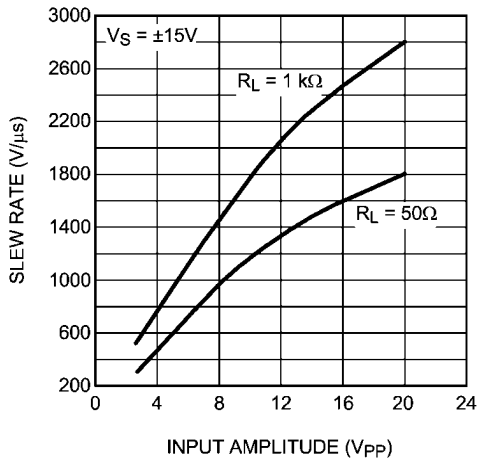
Slew Rate
