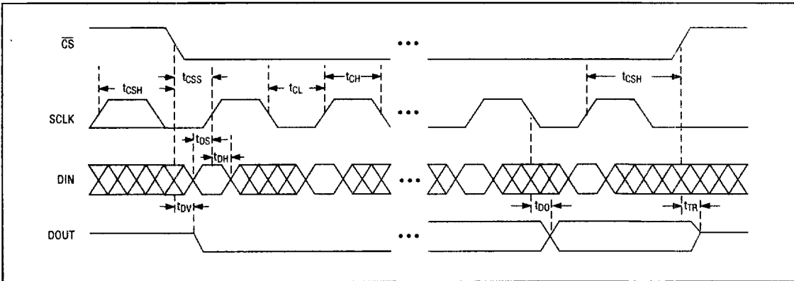
Figure 7. Detailed Serial-Interface Timing
