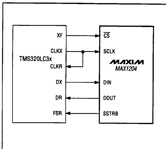
Figure 19. MAX1204 to TMS320 Serial Interface
