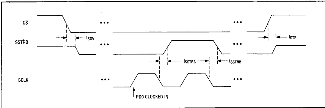
Figure 8. External Clock-Mode SSTRB Detailed Timing
