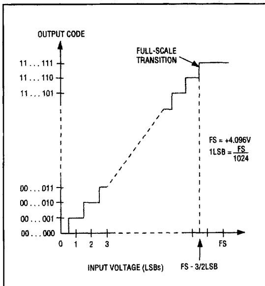
Figure 15. Unipolar Transfer Function, 4.096V = Full Scale
