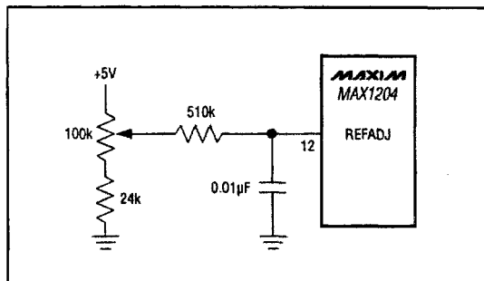
Figure 17. Reference-Adjust Circuit
