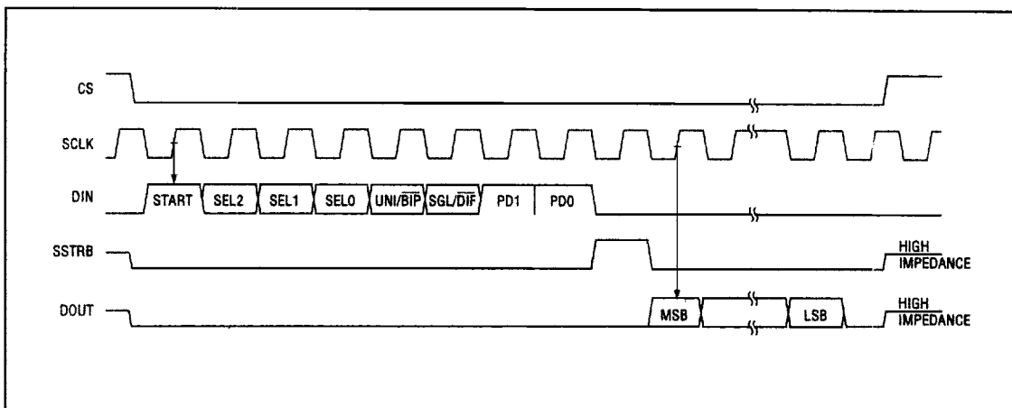
Figure 20. TMS320 Serial-Interface Timing Diagram
