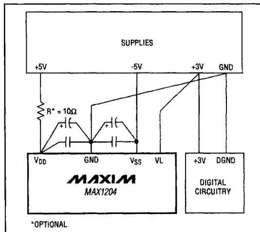
Figure 18. Power-Supply Grounding Connection
