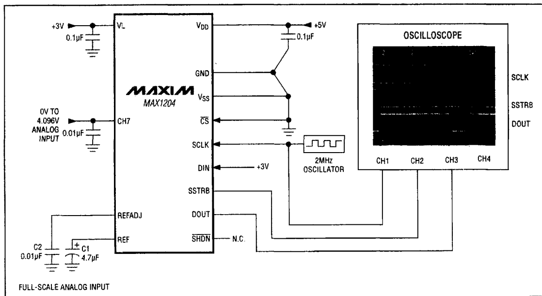
Figure 5. Quick-Look Circuit
