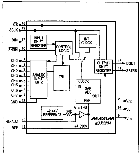
Figure 3. Block Diagram
