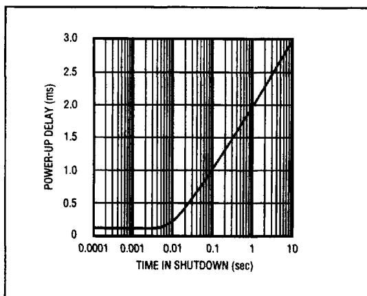
Figure 14c. Typical Power-Up Delay vs. Time in Shutdown
