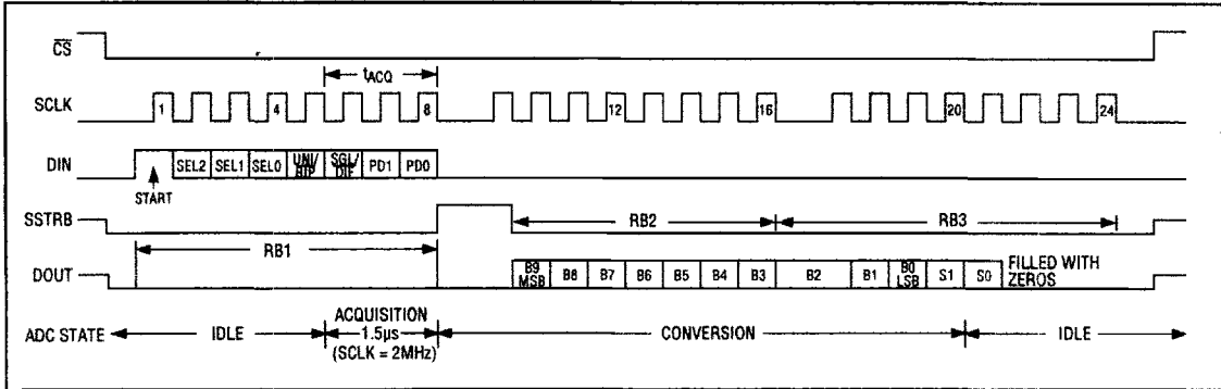
Figure 6. 24-Bit External-Clock-Mode Conversion Timing (Microwire/SPI Compatible)
