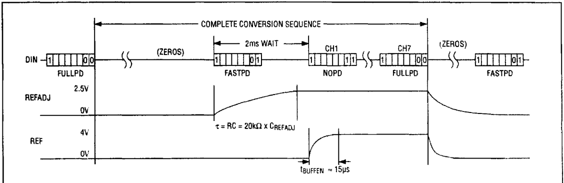
Figure 13. MAX1204 FULLLPD/FASTPD Power-Up Sequence
