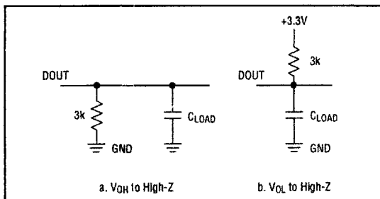
Figure 2. Load Circuits for Disable Time
