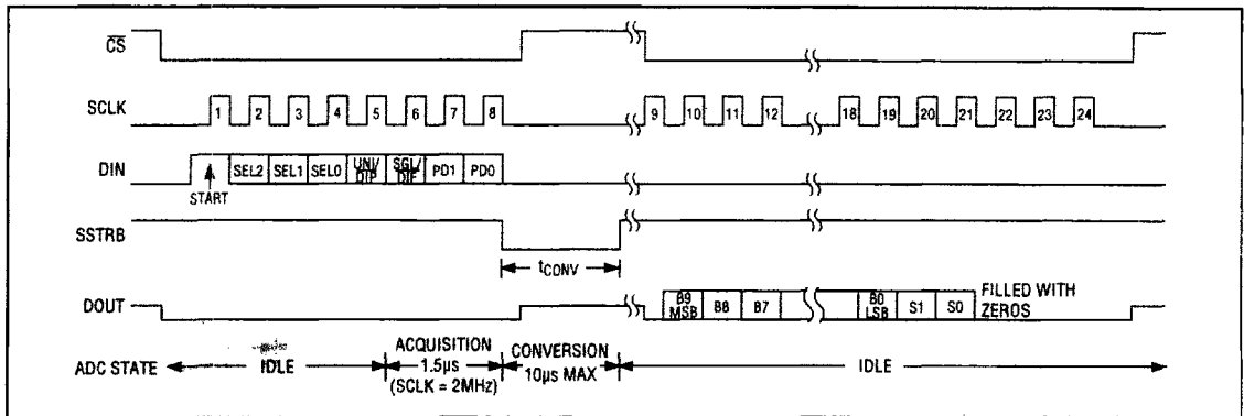
Figure 9. Internal Clock Mode Timing
