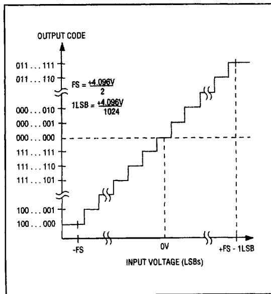
Figure 16. Bipolar Transfer Function, \pm 4.096V/2 = Full Scale
