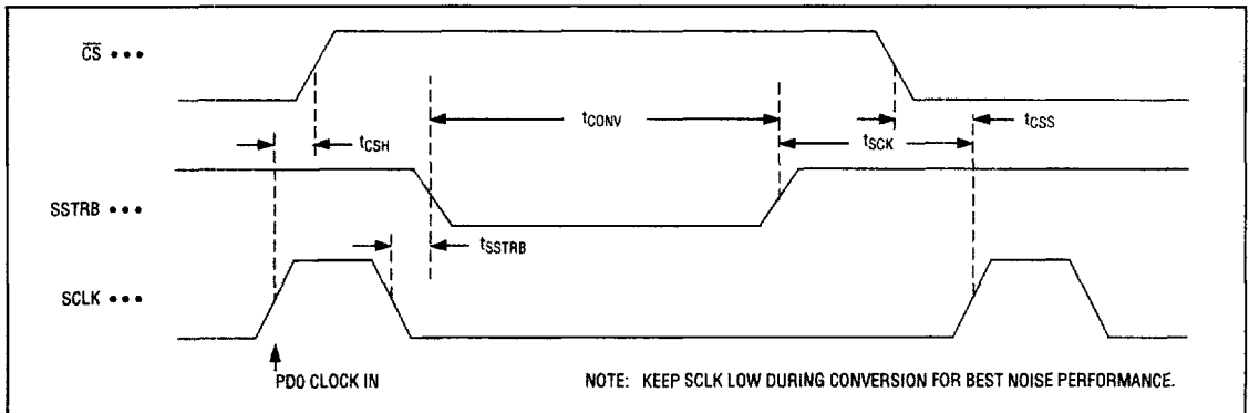
Figure 10. Internal Clock Mode SSTRB Detailed Timing
