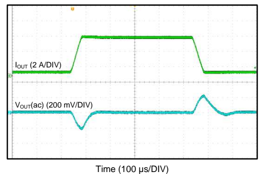
Figure 25. DCM Mode
