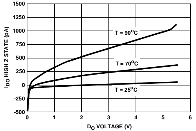
FIGURE 4. I_{DO} HIGH Z STATE vs D_0 VOLTAGE
