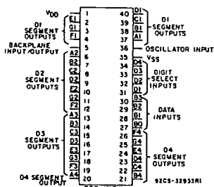
TOP VIEW TERMINAL ASSIGNMENT CD7211, CD7211A
