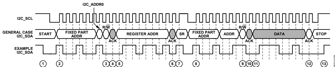
Figure 30. I 2 C Read Diagram
