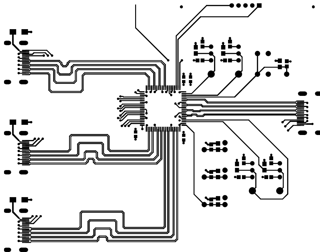
Figure 31. Layout of the TMSD Traces on the ADV3000 Evaluation Board (Only Top Signal Routing Layer is Shown)
