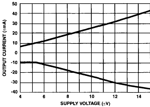
FIGURE 12. OUTPUT CURRENT vs SUPPLY VOLTAGE
