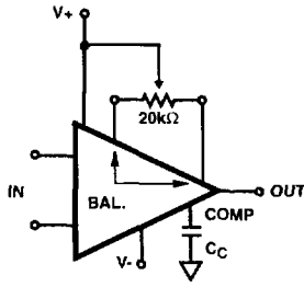
FIGURE 5. SUGGESTED V_{OS} ADJUSTMENT AND COMPENSATION HOOK-UP
