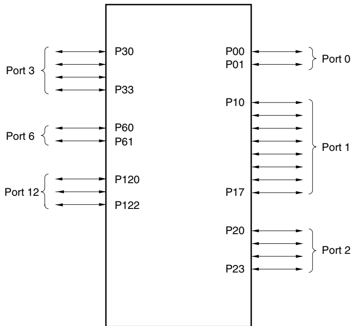
Figure 5-1. Port Types
