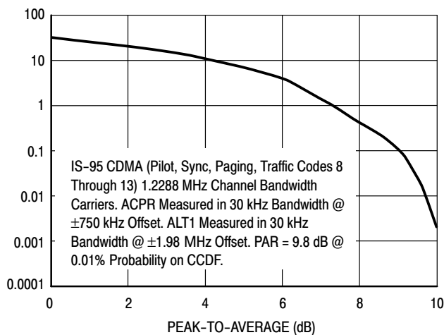
Figure 13. Single-Carrier CCDF N-CDMA
