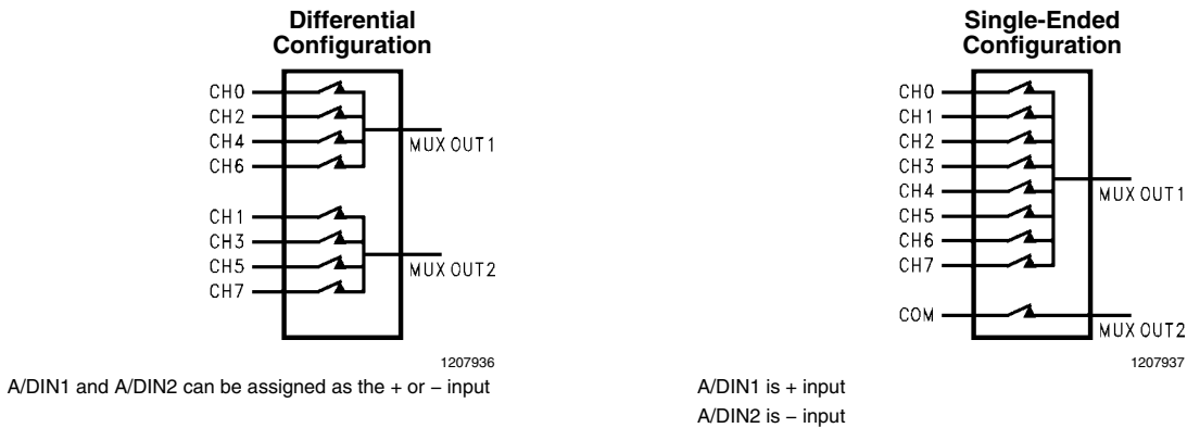
FIGURE 10. MUXOUT connections for multiplexer option
