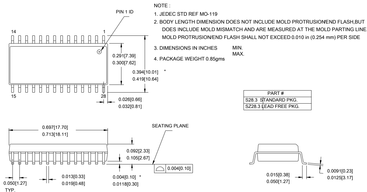
Figure 24. 28-Pin (300-Mil) Molded SOIC
