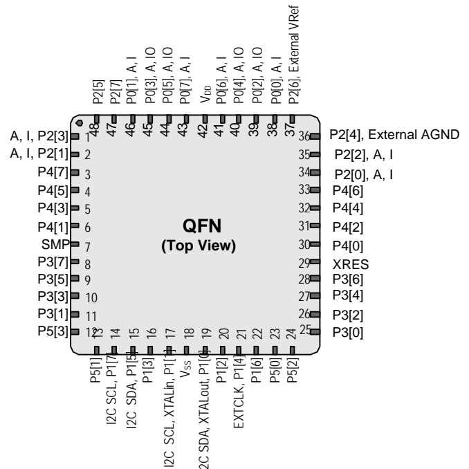
Figure 8. CY8C27643 48-Pin PSoC Device [9]
