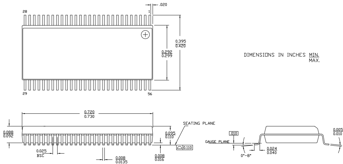
Figure 29. 56-Pin (300-Mil) SSOP
