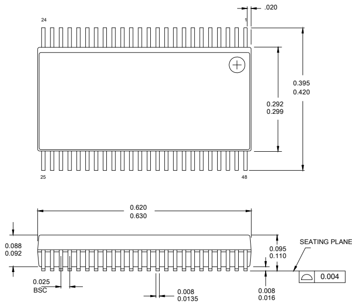
Figure 26. 48-Pin (300-Mil) SSOP
