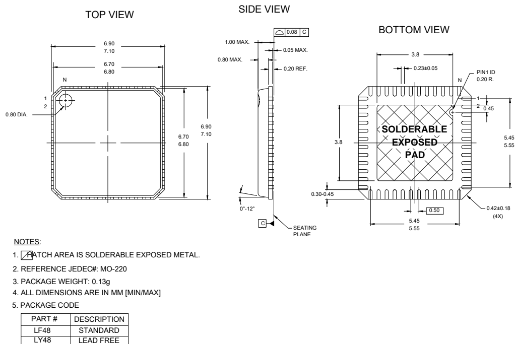
Figure 28. 48-Pin (7 × 7 mm) QFN
