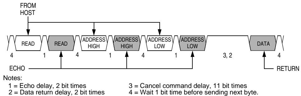
Figure 13-10. Read Transaction
