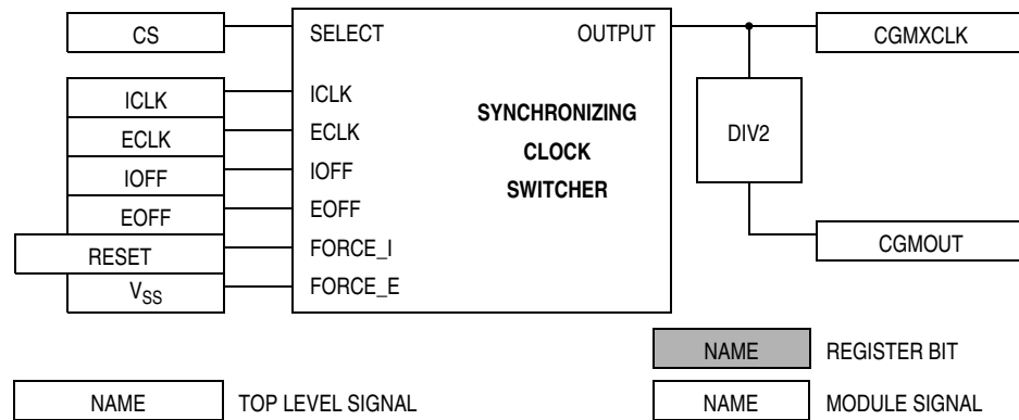
Figure 6-5. Clock Selection Circuit Block Diagram
