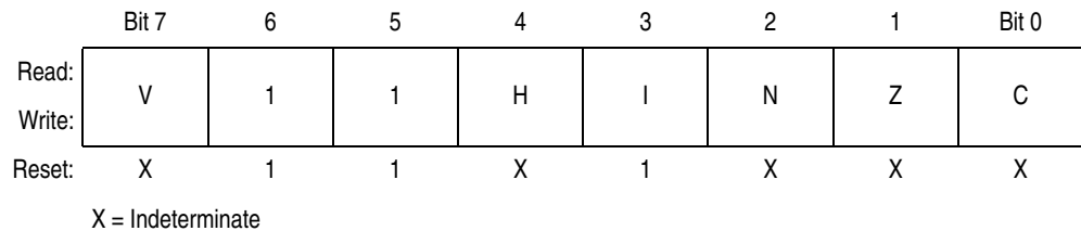
Figure 5-6. Condition Code Register (CCR)
