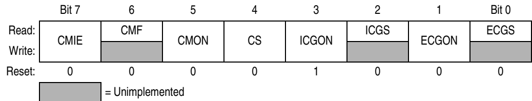
Figure 6-11. ICG Control Register (ICGCR)
