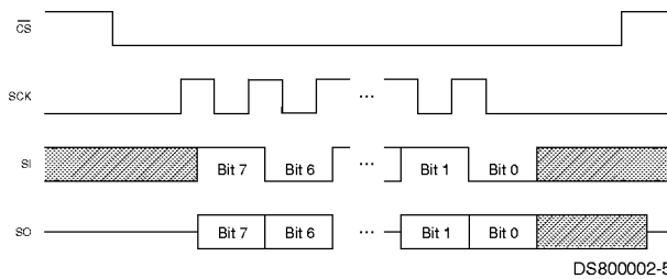
FIGURE 3. SPI Protocol
