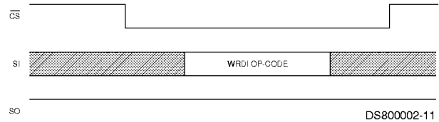
FIGURE 8. Write Disable
