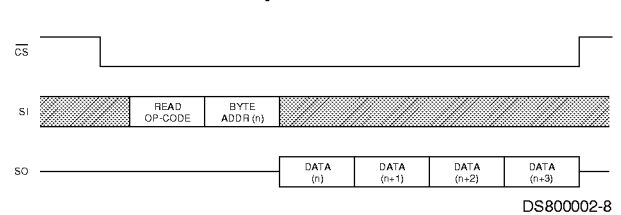
FIGURE 5. Read Sequence
