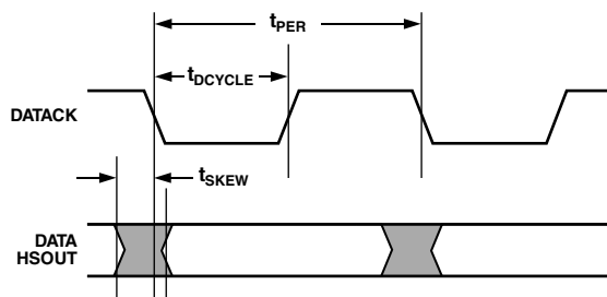
Figure 7. Output Timing
