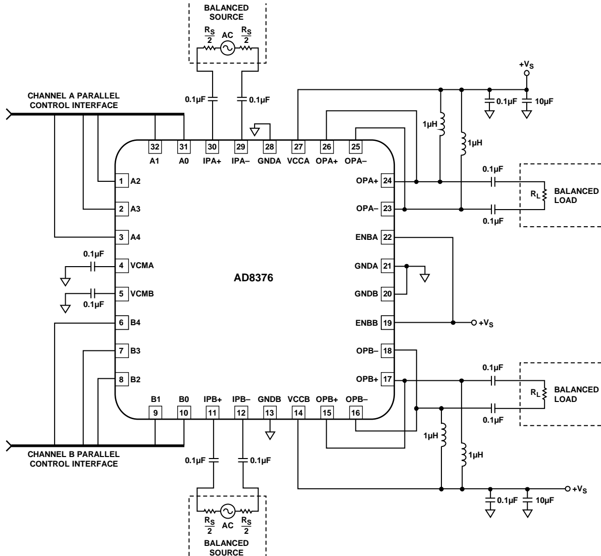
Figure 36. Basic Connections
