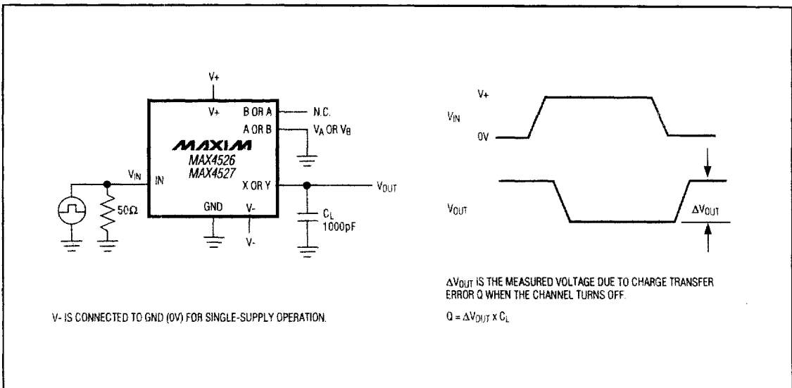
Figure 5. Charge Injection
