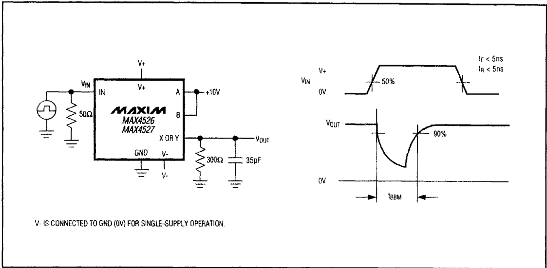
Figure 4. Break-Before-Make Interval
