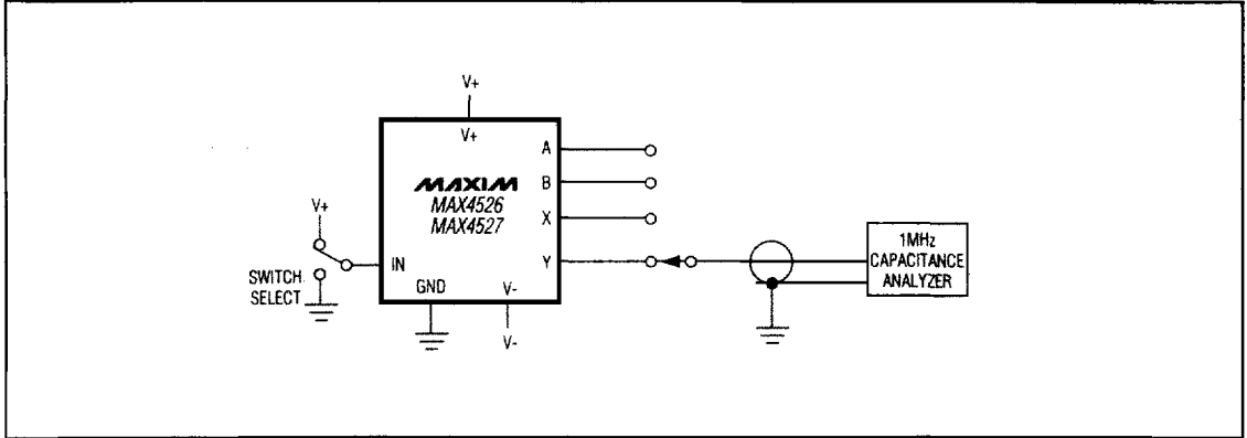
Figure 6. A, B, X, Y Capacitance
