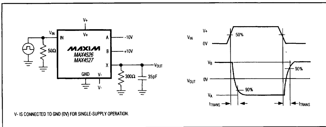
Figure 3. Address Transition Time
