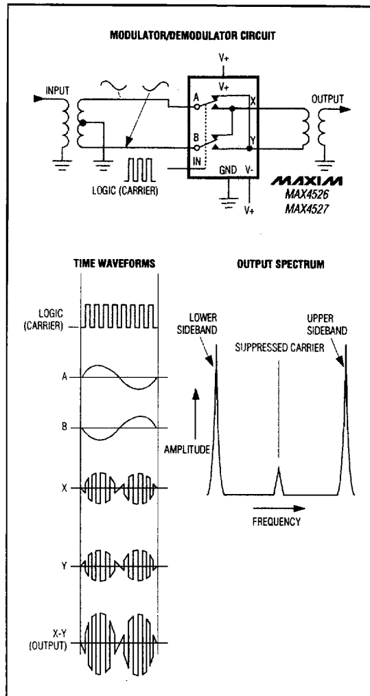
Figure 2. Balanced Modulator/Demodulator
