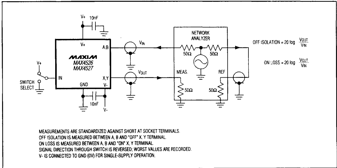
Figure 7. Off Isolation and On Loss
