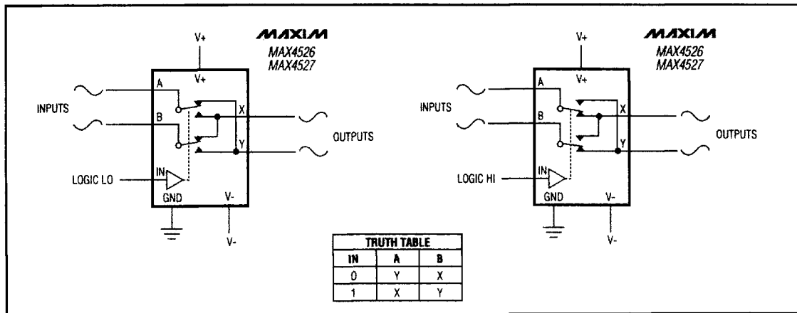
Figure 1. Typical Application Circuits
