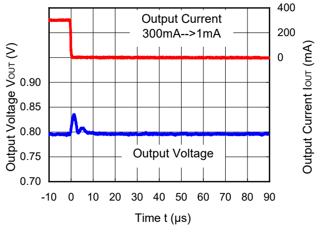
RP505K081A/B ( V_{IN}=3.6V )
