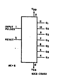
Fig. 2 - Functional diagram for CD4024AT.
