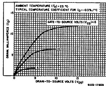
Fig. 3 - Typical output n-channel drain characteristic.
