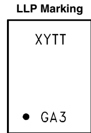
Top View XY - Date Code TT - Die Traceability G - Boomer Family A3 - LM4902LD
