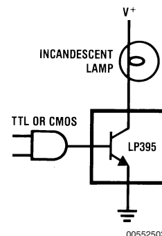
Fully Protected Lamp Driver
