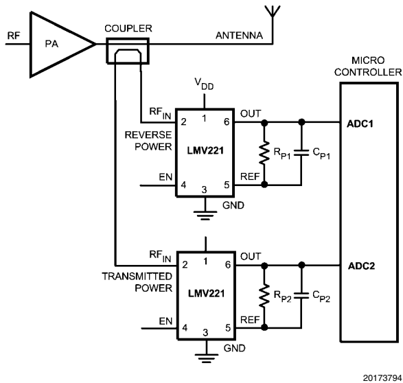
FIGURE 4. VSWR Application
