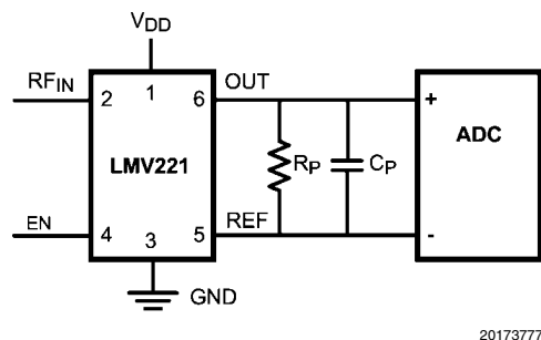
FIGURE 12. Single Ended and Differential Application
