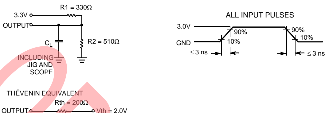
Figure 4. AC Test Loads and Waveforms [9, 10]
