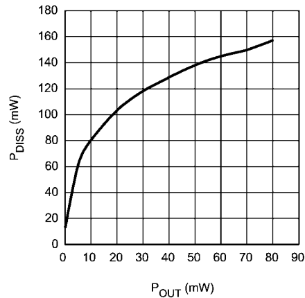
LM4844TL Power Dissipation vs Output Power V_{DD} = 5V, R_L = 8\Omega OCL HP, per channel
