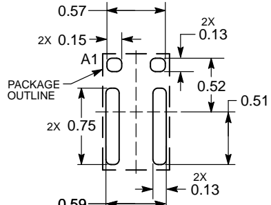
DIMENSIONS: MILLIMETERS
