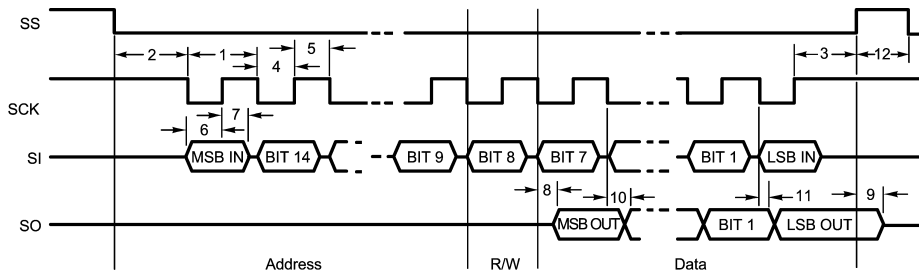
FIGURE 4. SPI Timing Diagram
