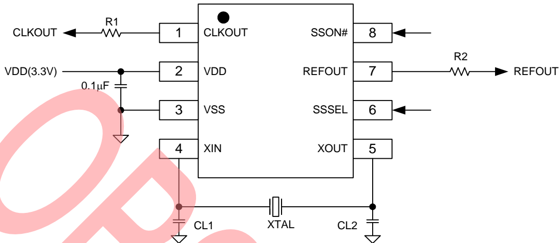
Figure 3. Application Schematic
